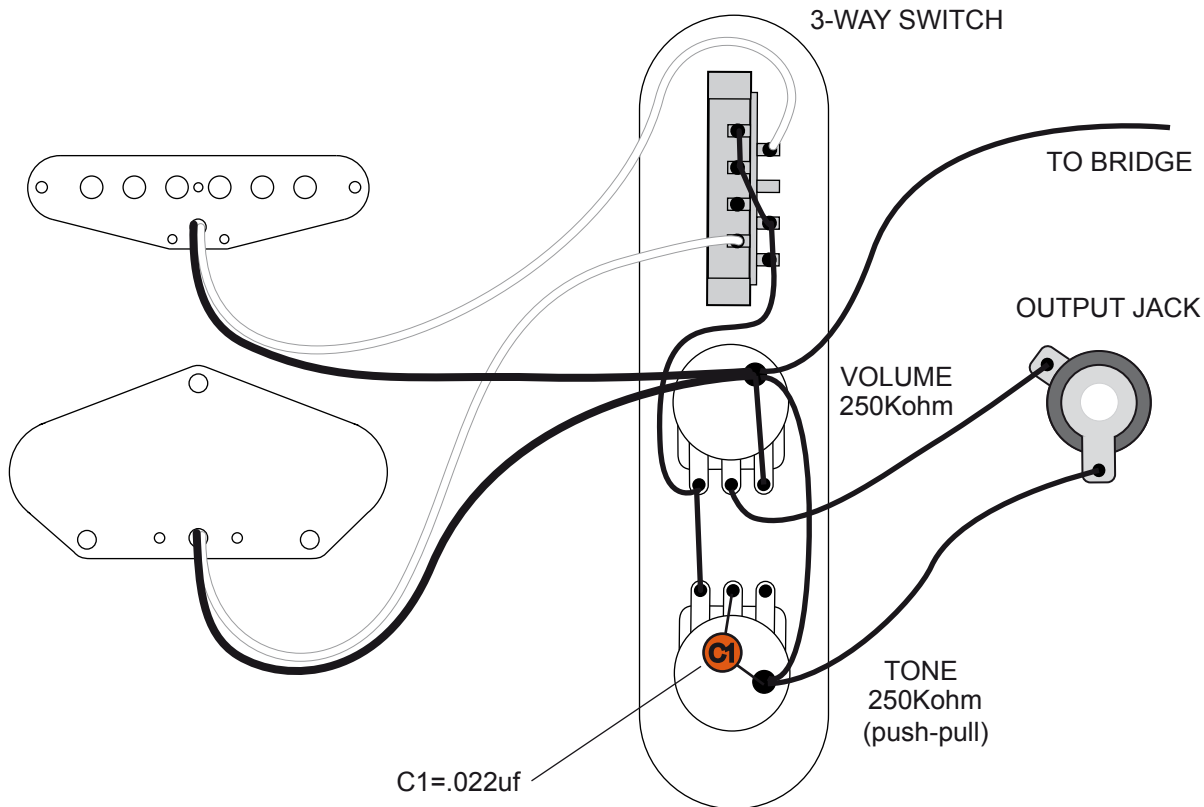
SINGLE COIL+SINGLE COIL Volume, Tone, 3-way switch
