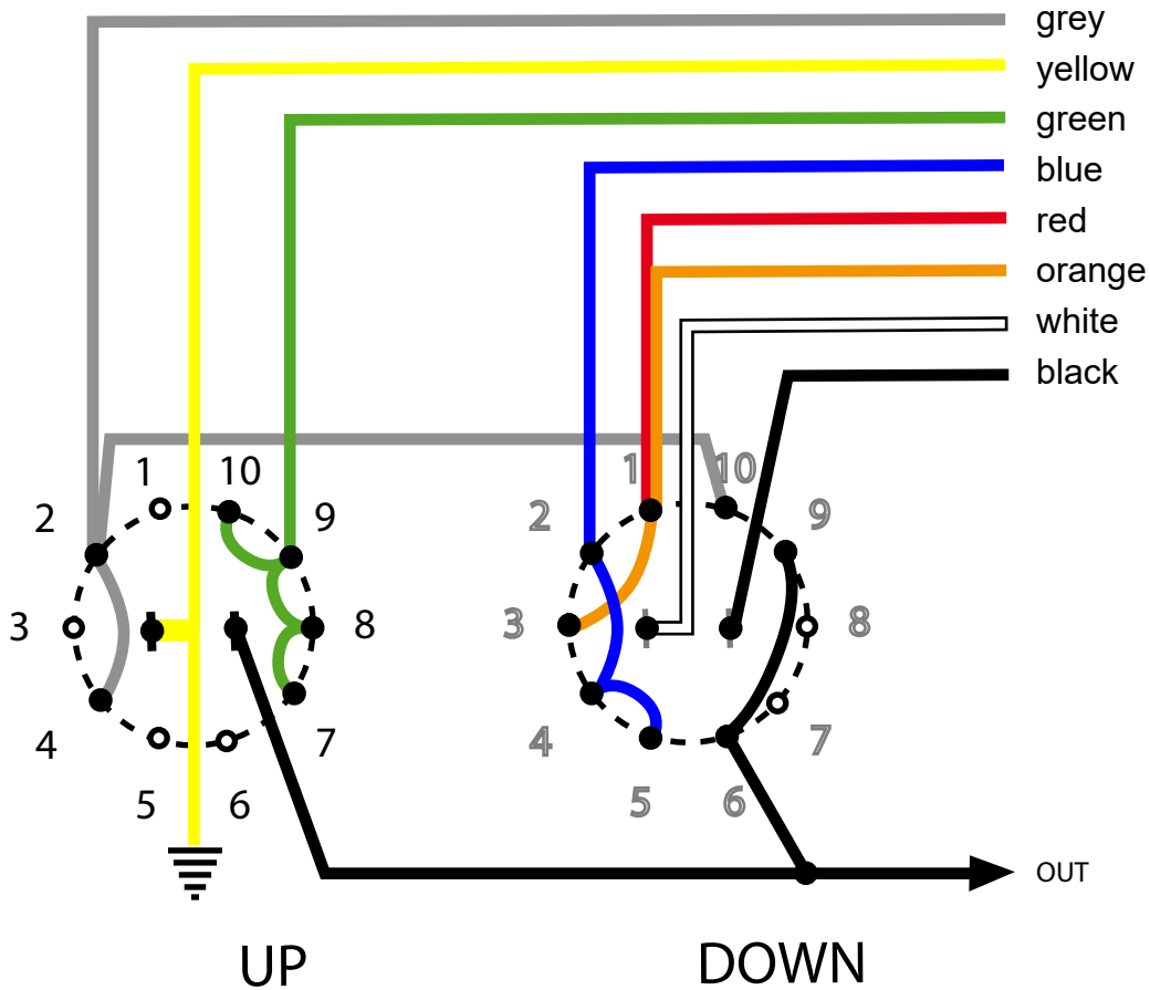
1 - JAZZ BASS bridge side
