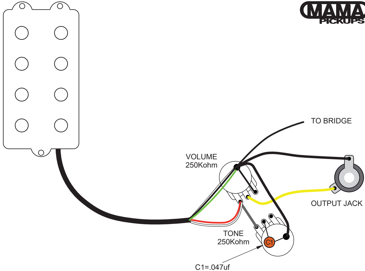
MUSIC MAN® (parallel wiring) Volume, Tone
