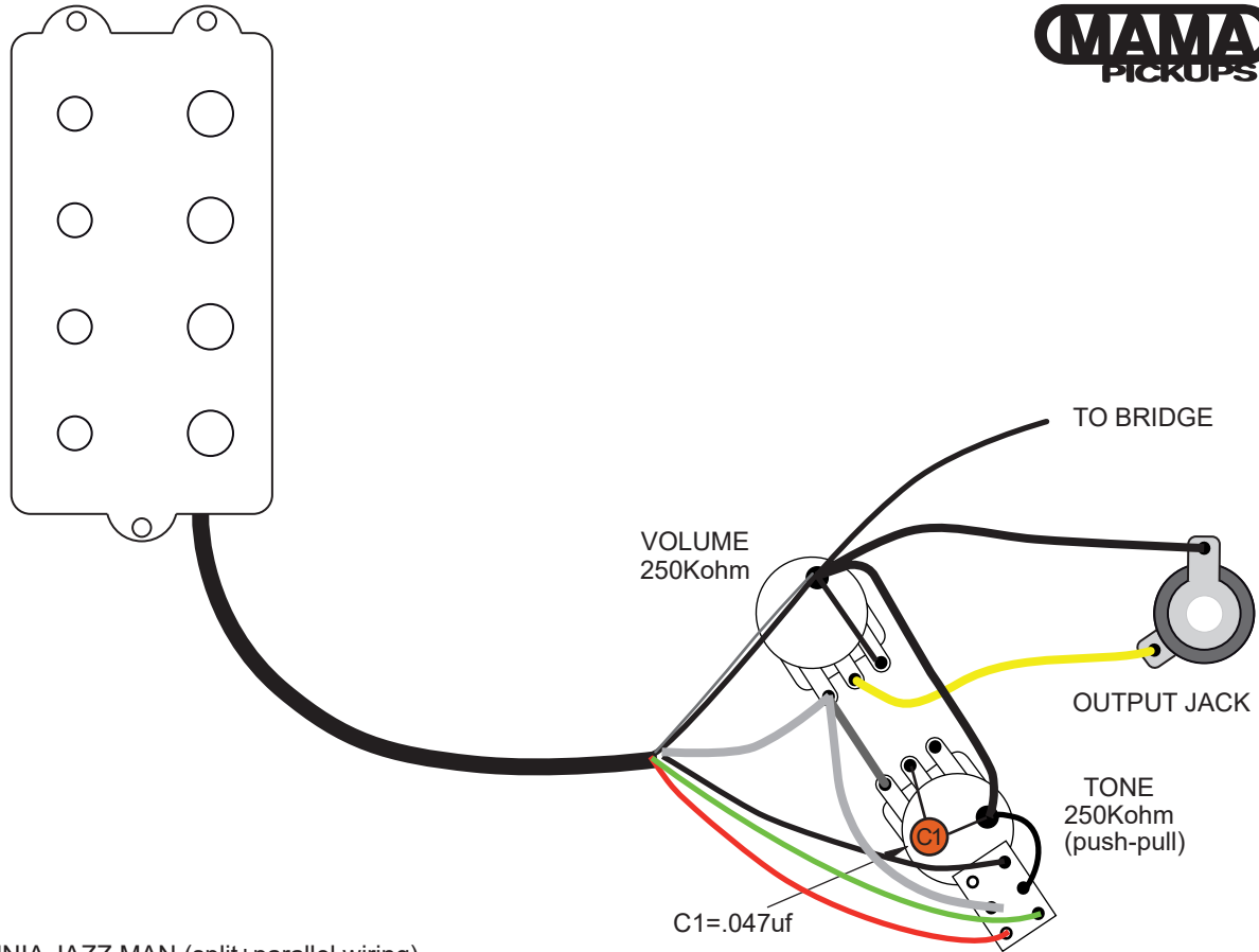
OMNIA JAZZ MAN (split+parallel wiring) Volume, Tone, Push-Pull
