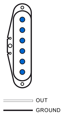
REVERSE (RWRP) STRATO
