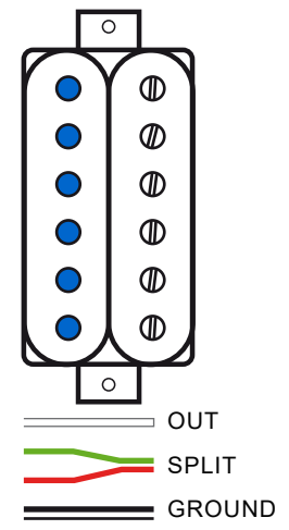
OMNIA NECK HUMBUCKER
