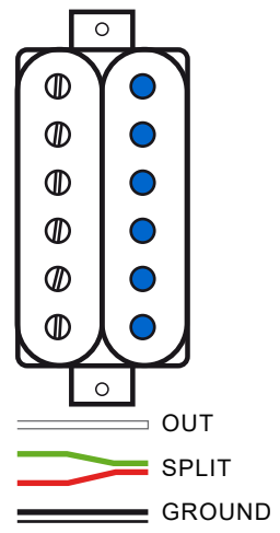
4-CONDUCTOR HUMBUCKER
