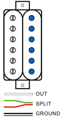
4-CONDUCTOR HUMBUCKER
