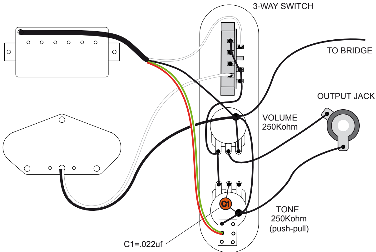
SINGLE COIL+HUMBUCKER Volume, Tone, 3-way switch
