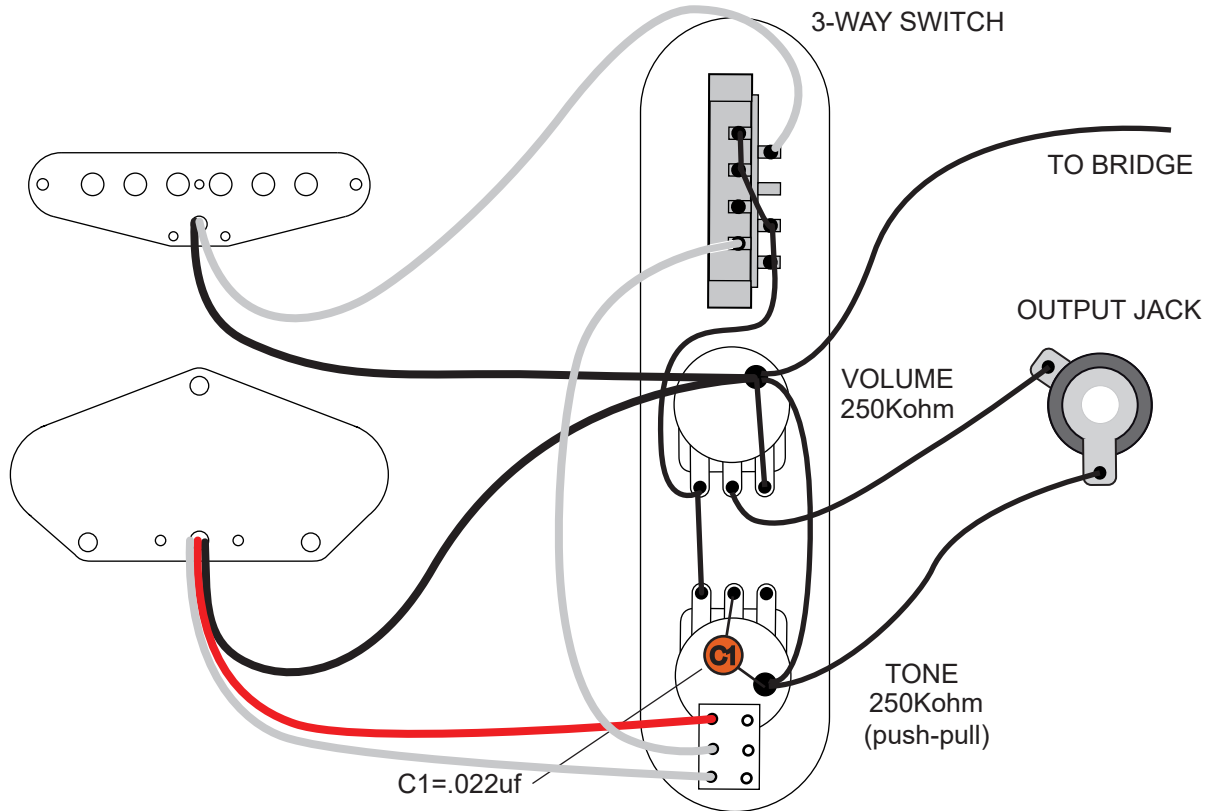
SINGLE COIL+T-RUNNER TAP Volume, Tone, 3-way switch, push-pull
