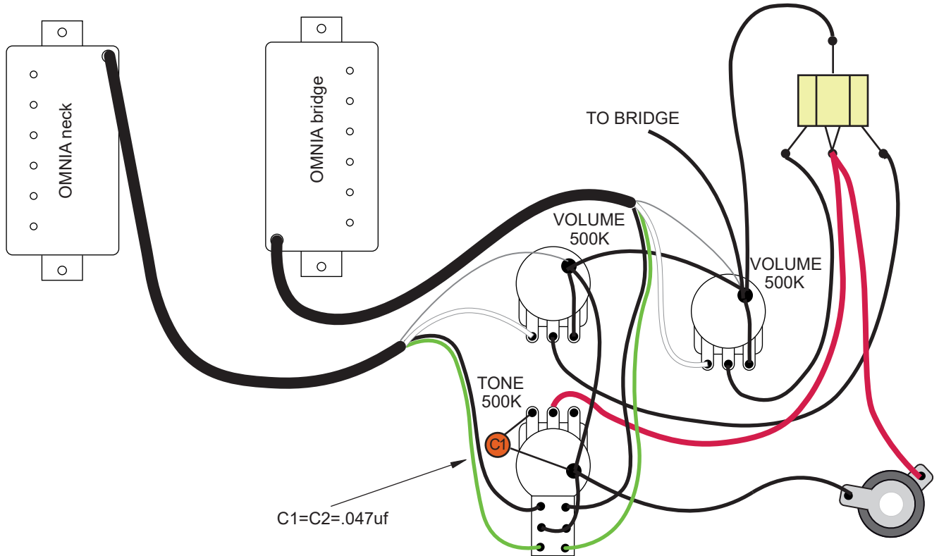
OMNIA+OMNIA Volume, Volume, Tone, 3 way toggle switch, push-pull (splt)
