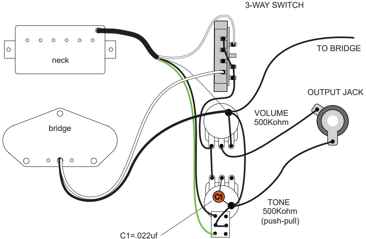
SINGLE COIL+OMNIA 3-way switch, Volume, Tone, push-pull
